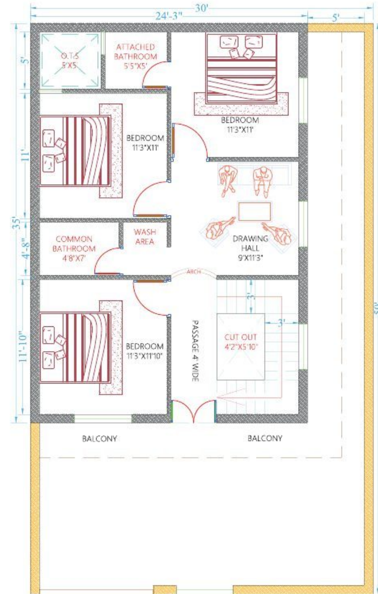
FIRST FLOOR
